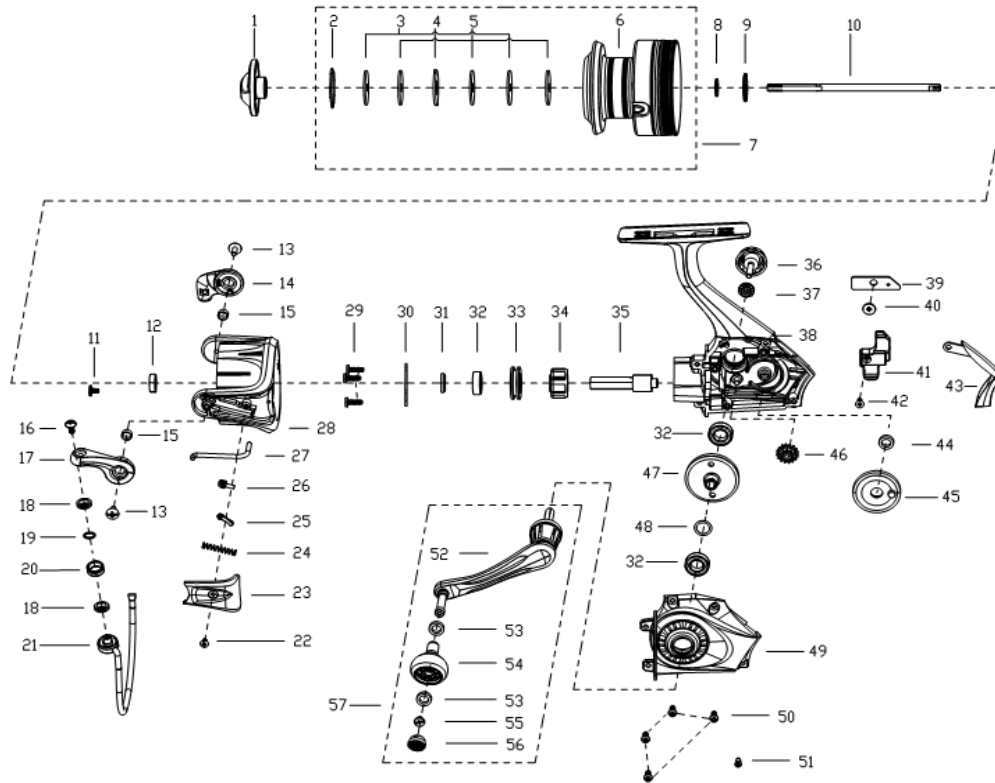
PARTS LIST OF MAXXSP 60
